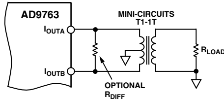
Figure 16. Differential Output Using a Transformer
